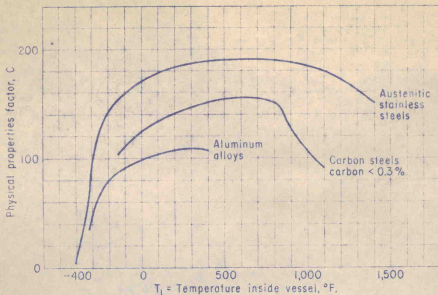
Temperature-dependent physical-property factor C for stainless and carbon steels and aluminum alloys; used in Eqs. (1) and (2).—Fig 2
