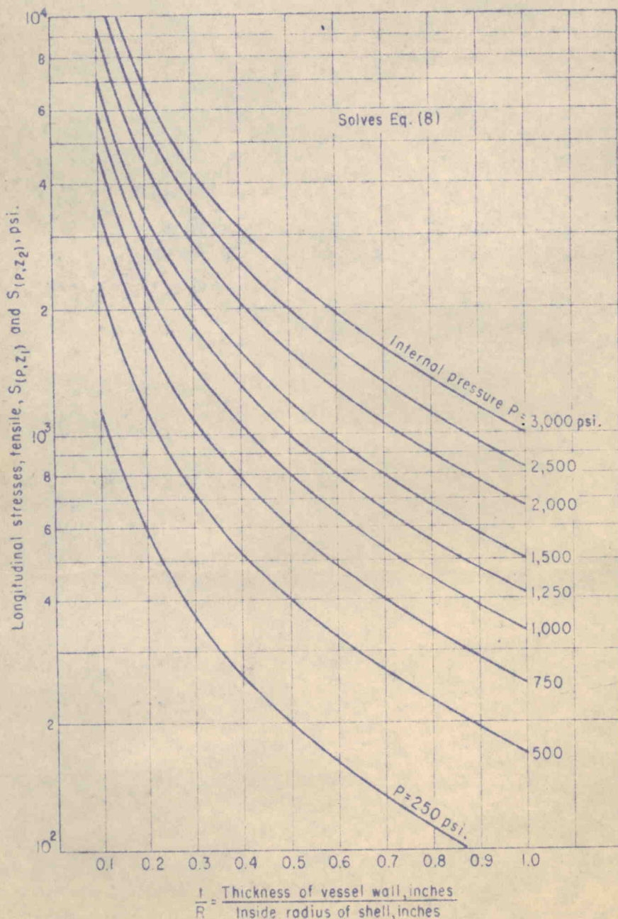
Longitudinal shell stresses, assumed constant throughout the thickness, in thick-walled vessels subjected to internal pressure; solves Eq. (8).—Fig. 6
