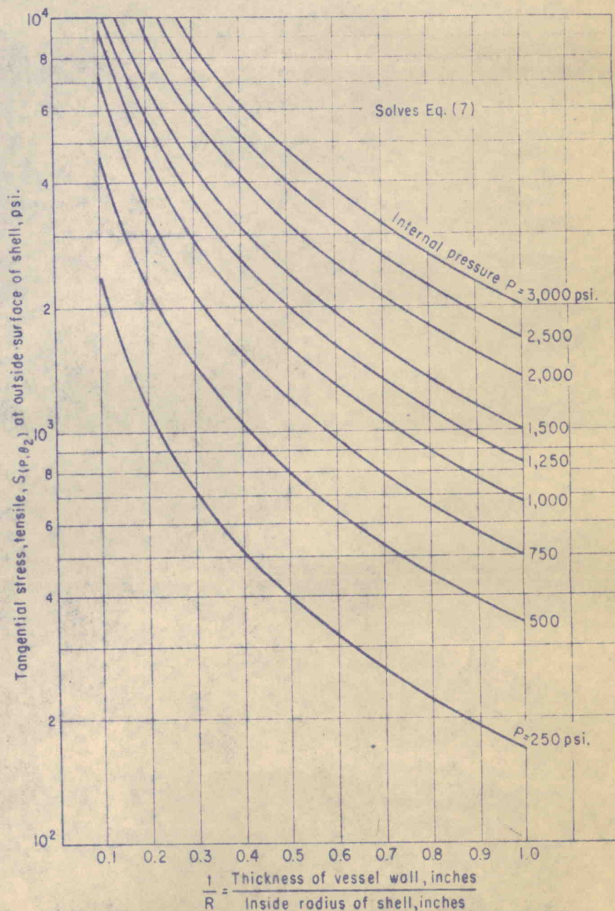
Tangential stresses in the outer surface of a thick-walled vessel subjected to internal pressure; solves Eq. (7).—Fig. 5
