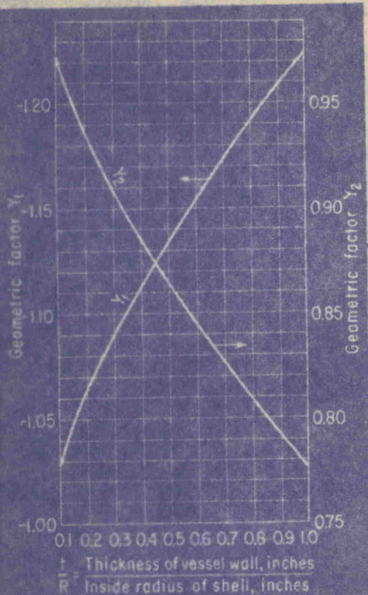
Dimensionless geometric factors Y_1 and Y_2 for cylindrical shells of varying t/R ratio; used in Eqs. (1) and (2).—Fig. 3
