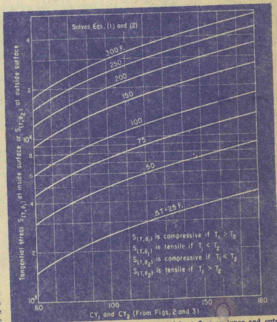
Steady-state thermal stresses under isothermal heat flow on inner and outer surfaces of a thick-walled shell; solves Eqs. (1) and (2).—Fig. 1
