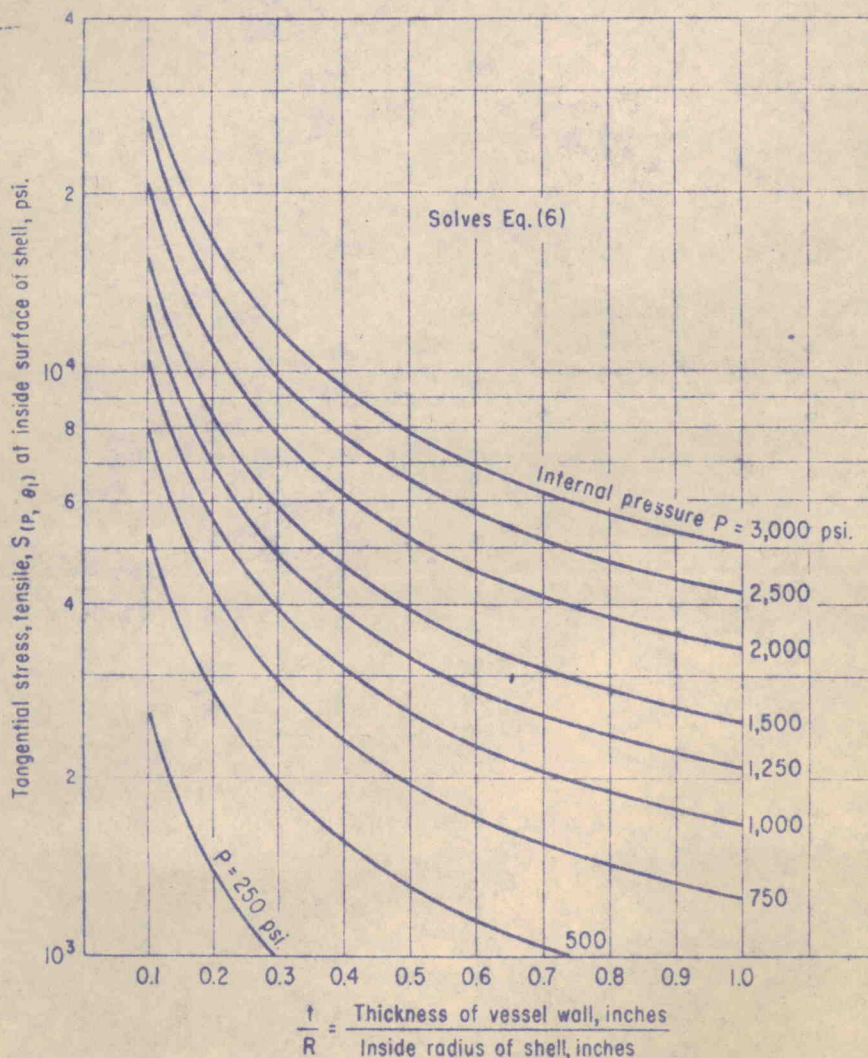
Tangential stresses in the inner surface of a thick-walled vessel subjected to internal pressure; solves Eq. (6)—Fig. 4
